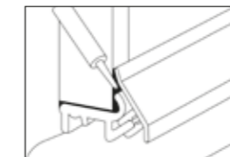
Seal two Panel encapsulated in sealant.
